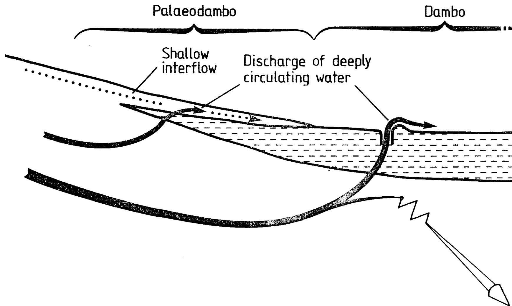
Figure 7.3 Groundwater circulation in vicinity of a dambo.
