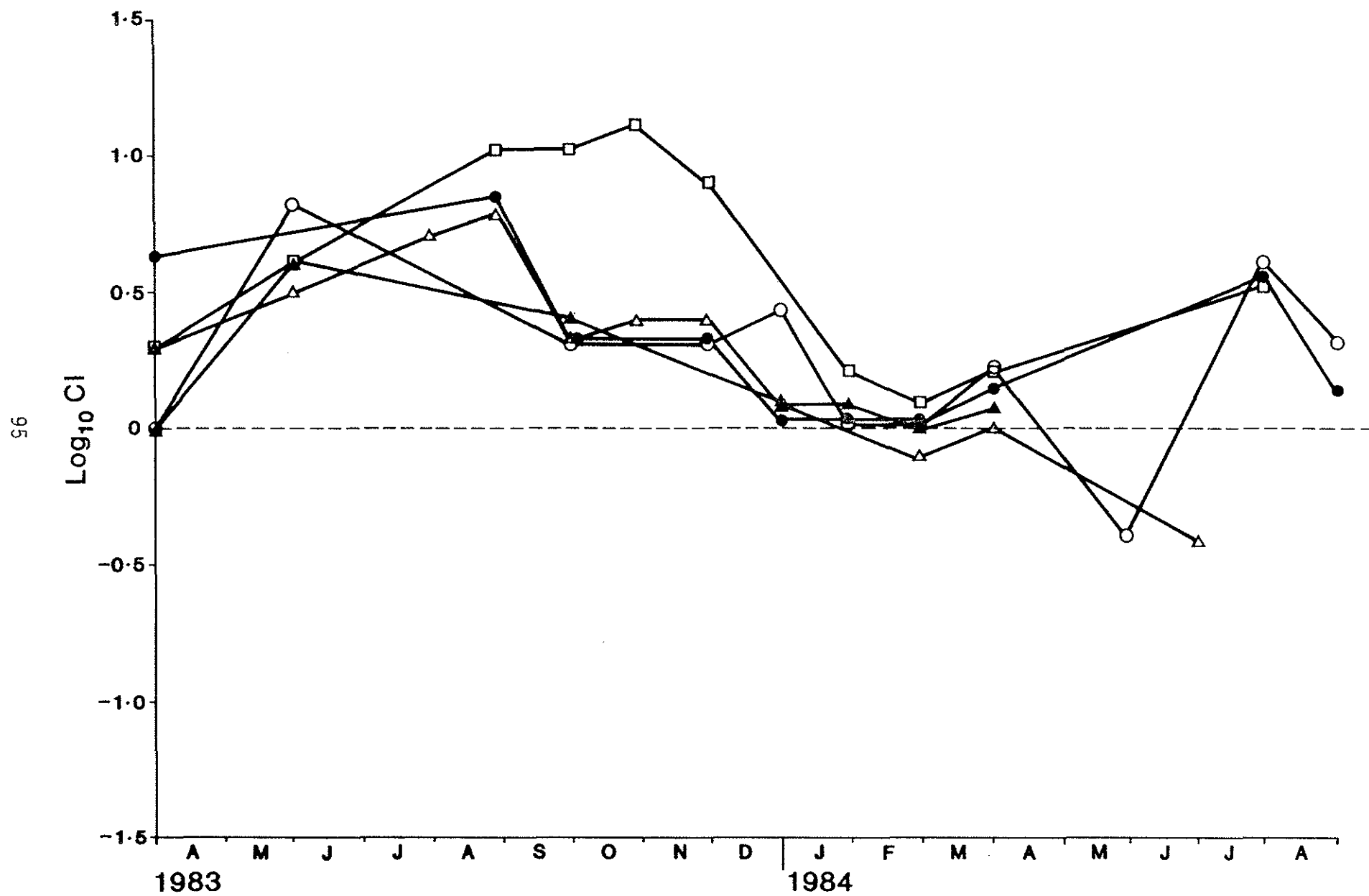
Figure 11.2 Chloride content of surface runoff in 4 further catchments overlying basement rocks in central plateau region of Malawi.
