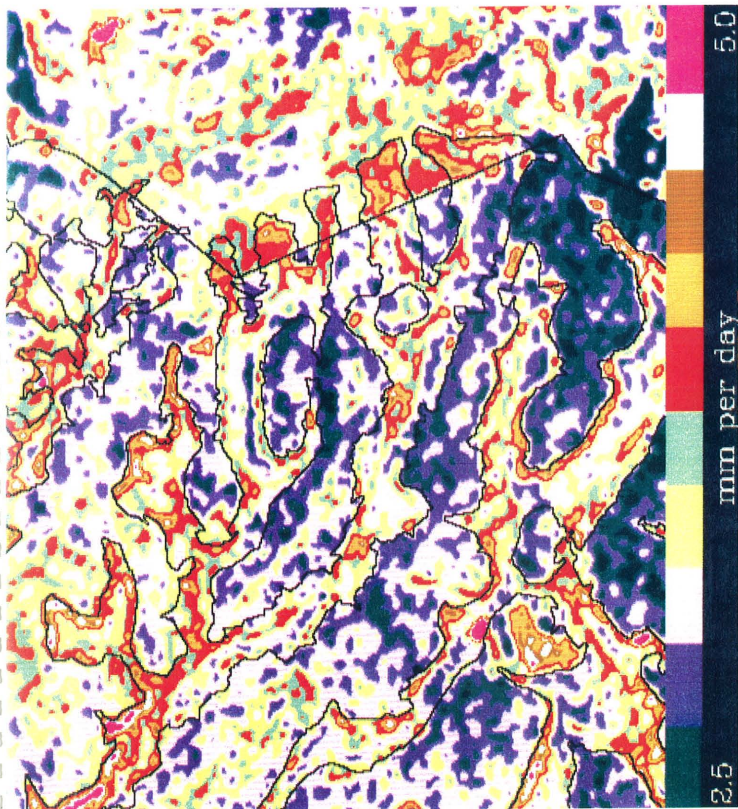
Figure 8.7 The evaporation expressed in \text{mm day}^{-1} over the 15 by 15 km area.
