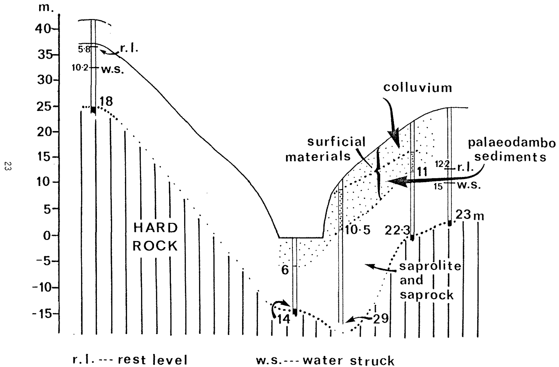
Figure 5.3 Geological cross-section at Chikobwe dambo.
