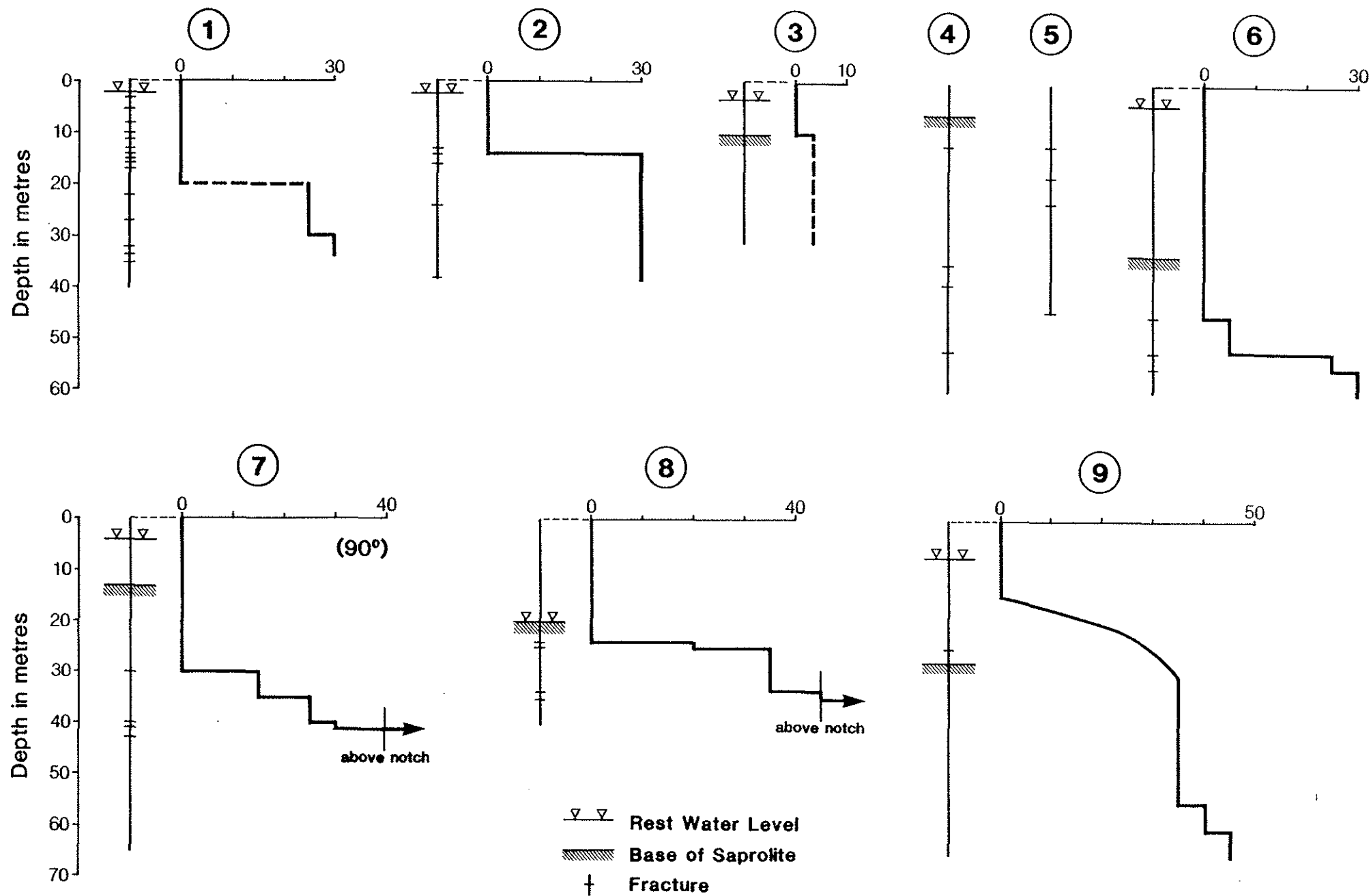
Figure S11. Drilling Discharge in mm over V Notch (45° or 90°, when shown) (Data from BGS test drilling programme)
