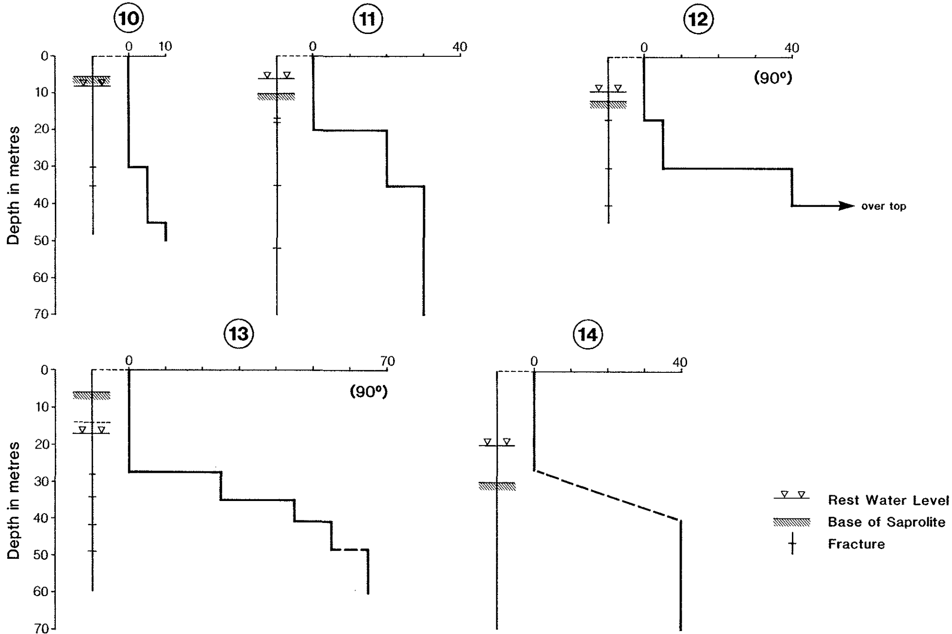
Figure 11.11 Drilling Discharge in mm over V Notch (45° or 90°, when shown) Data from BGS Drilling Programme - 10 Mhatiwa Inclined, 11 Mhatiwa V., 12 Rungai, 13 Chikofa, 14 Sarahuru.
