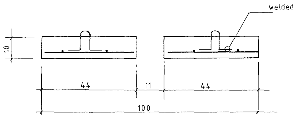
Section X X scale 1: 10
