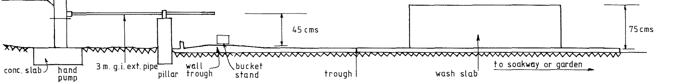
Side View Fig. D. 8.1. TYPICAL HANDPUMP INSTALLATION IN MALAWI
