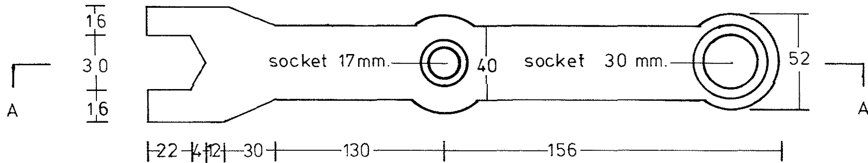
PLAN VIEW.
