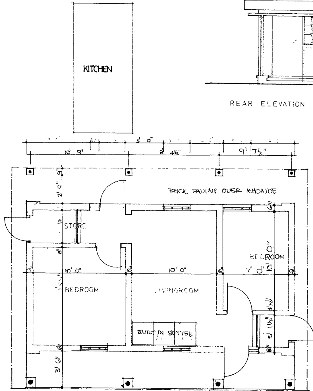
Figure D.10.2. Plans for Low-cost House
