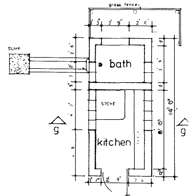
kitchen - bath plan
