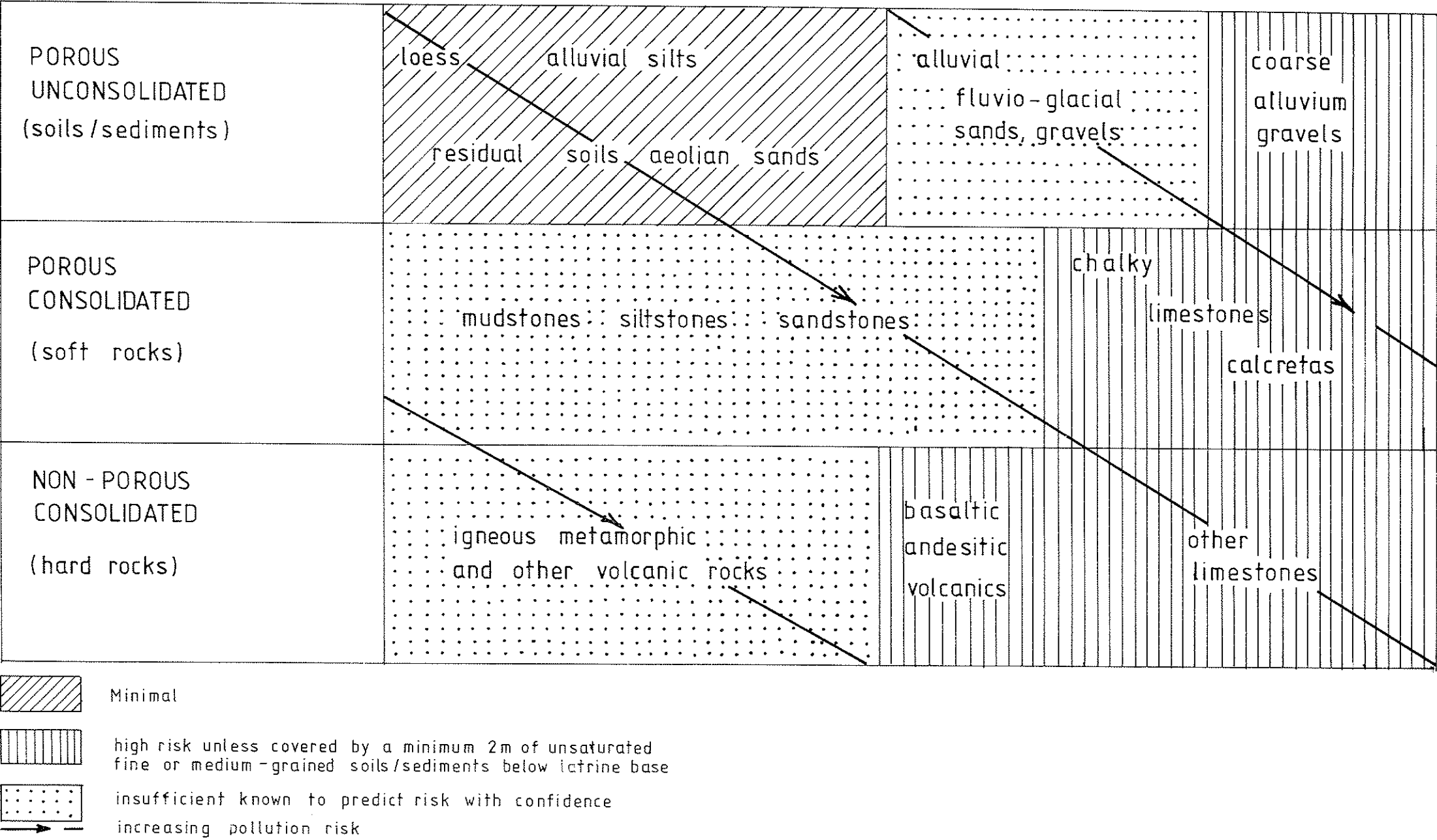
Figure D.16.1 CLASSIFICATION OF SOILS AND ROCKS IN AN ARRAY OF RELATIVE POLLUTION RISK (after Lewis et al, 1982)
