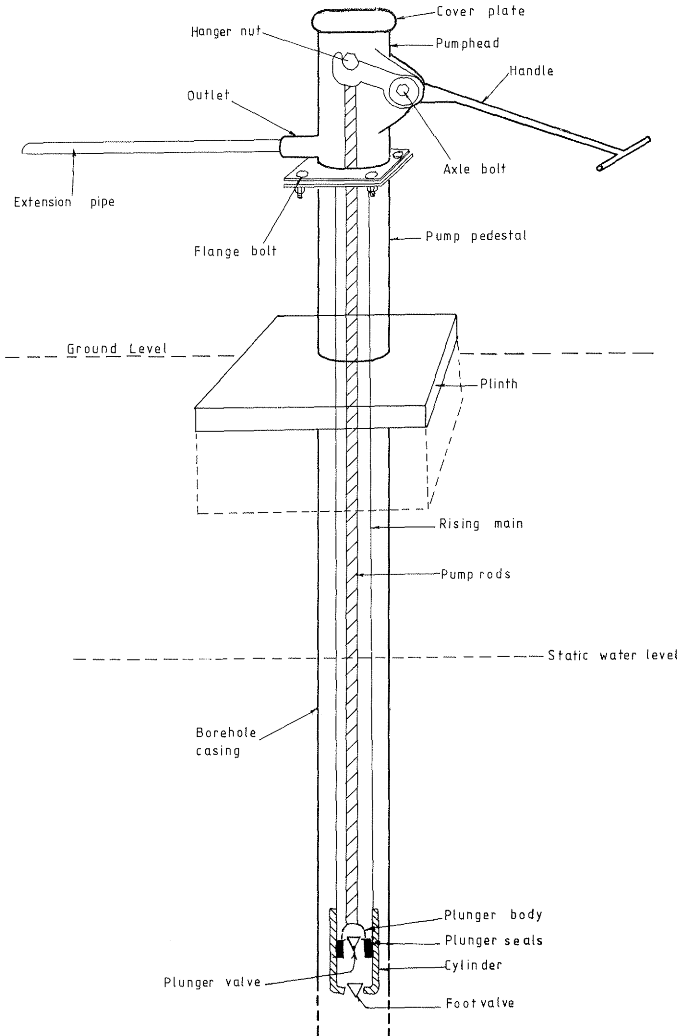
Figure D.7.1. COMPONENTS OF A HANDPUMP (Borehole)
