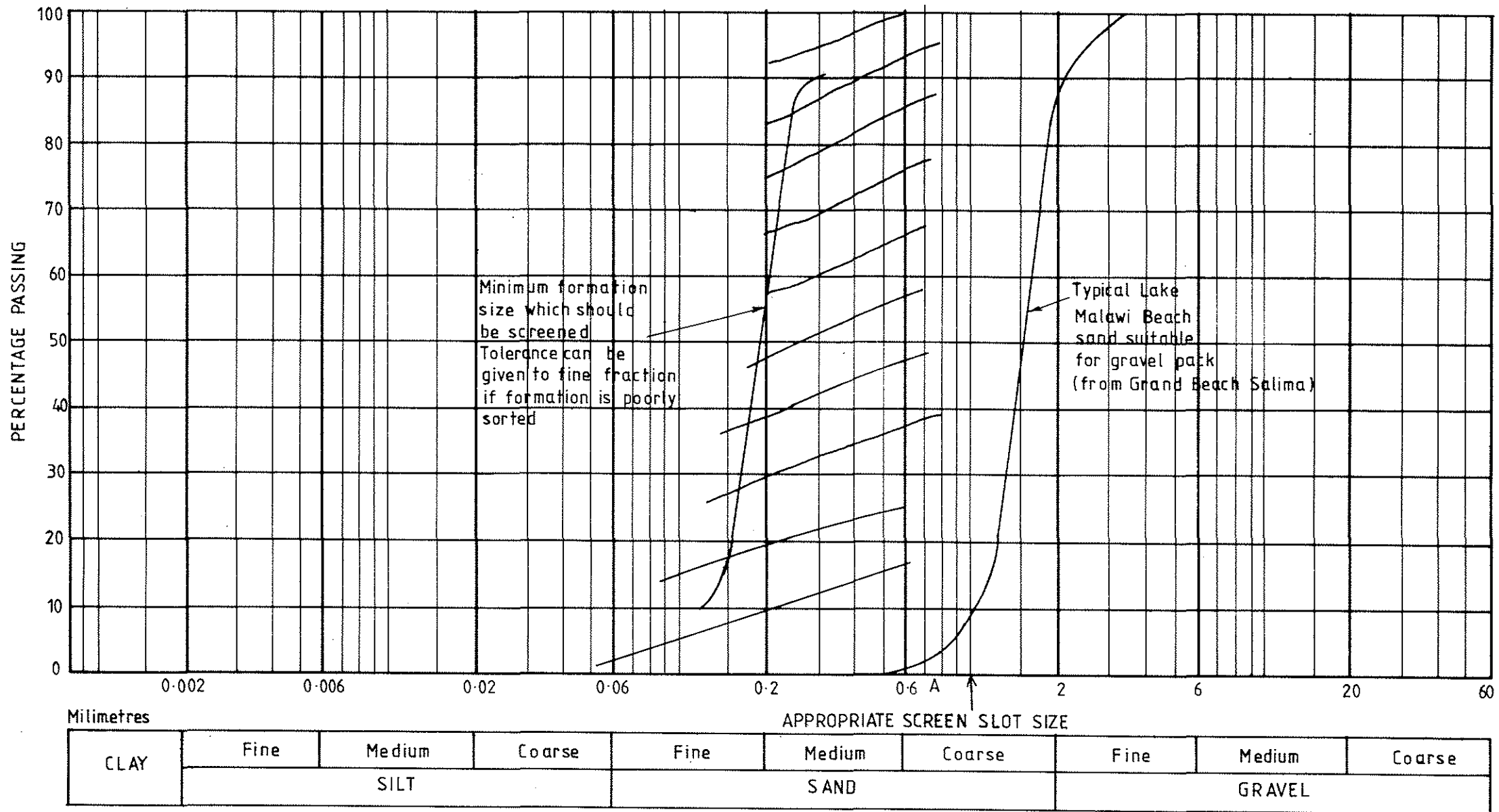
Figure D.3.4. FORMATION AND GRAVEL PACK GRADING CURVES
